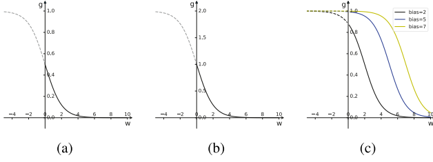
Fig. 3. Function study for DDI gating mechanism. Since W_{i,j}^{DDI} \geq 0 , the dotted line in the graph is the point that the function cannot get. Function images with different bias values is shown in subgraph (c). It can be seen that the value of g is more flexible and the expression ability of the model is stronger. (a) g = 1 - \sigma(W^{DDI}) . (b) g = 2(1 - \sigma(W^{DDI})) . (c) g = 1 - \sigma(W^{DDI} - B^{DDI}) .
