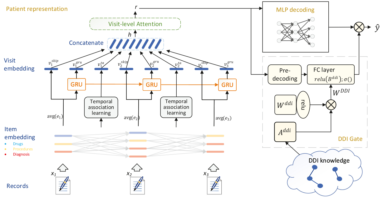
Fig. 1. Drug recommendation model based on message propagation network and DDI gating mechanism. (1) The patient presentation module contains three sub-modules. (a) Temporary association learning. The patient's visit records are regarded as a temporal graph. KGAT [20] which is a message propagation network is used to learn message propagation in the temporal graph. (b) Skip GRU is used to learn visits' representation. (c) Visit-level attention is used to obtain the patient representation. (2) The DDI gating module generates a gate vector to control the final output of the model. To obtain the interpretable DDI intensity, the weight parameter is set to not less than 0. (3) An MLP decoding module is used to predict drug combinations. The decoding module is extended to BNN, so that the model can output a variety of drug combinations and give the corresponding confidence.
