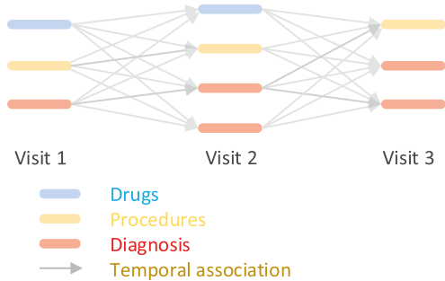
Fig. 2. Medical temporal graph. Each medical item in the medical visit is regarded as a node in the temporal graph. The relationship “temporal association” is built between two medical items from adjacent visits. The importance of “temporal association” depends on the learning of the message propagation neural network (e.g., KGAT [20]).
